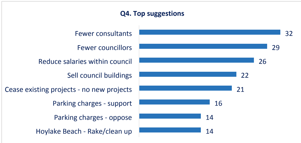
Figure 10: Top suggestions
